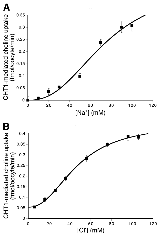
Fig. 4. Kinetic analysis of choline uptake mediated by hCMT1 in Xenopus oocytes. A: Effect of [\text{Na}^+] on CHT1-mediated choline uptake. The [\text{Na}^+] was varied between 0 and 100 mM, by replacing NaCl with LiCl. The data were fitted to the Hill equation. The choline uptake in oocytes injected with water was subtracted from that in oocytes injected with cRNA, yielding hCMT1-mediated choline uptake. B: Effect of [\text{Cl}^-] on CHT1-mediated choline uptake. The [\text{Cl}^-] was varied between 6 and 106 mM, by replacing NaCl with NaI. The data was fitted to the Hill equation. The choline uptake in oocytes injected with water was subtracted from that in oocytes injected with cRNA, yielding hCMT1-mediated choline uptake.
